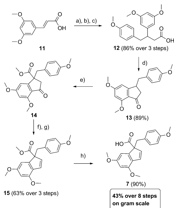
Scheme 2. Reagents and conditions: a) H 2 SO 4 (cat.), MeOH, 70 °C, 12 h; b) 4-MeOC 6 H 4 CH 2 MgCl (2.0 equiv), CuI (2.0 equiv), TMEDA (2.2 equiv), TMSCl (5.0 equiv), Et 2 O/THF, –78 °C/–20 °C, 3 h; c) NaOH (10%), MeOH, 70 °C, 2 h; d) MSA (10 equiv), 70 °C, 3 h; e) LDA (2.2 equiv), ClCO 2 Me (1.3 equiv), –78 °C/RT, 5 h; f) NaBH 4 (1.5 equiv), CeCl 3 (1.1 equiv), MeOH, 0 °C, 0.5 h; g) MsCl (2 equiv), NEt 3 (3 equiv), CH 2 Cl 2 , 0 °C, 17 h; h) NaOH (30%), EtOH/H 2 O (5:1), 5 °C, 16 h. MSA: methanesulfonic acid, LDA: lithium diisopropylamide, MsCl: methanesulfonyl chloride.
