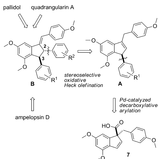
Scheme 1. Retrosynthesis of quadrangularin A ( 2 ), ampelopsin D ( 3 ), and pallidol ( 4 ).
