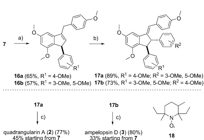
Scheme 3. Key steps in the modular approach to the natural products starting with rac - 7 (only one enantiomer drawn). Reagents and conditions: a) 7 (1.1 equiv for 16a , 1.3 equiv for 16b ), [Pd(dba) 2 ] (20 mol %), NaOtBu (1.1 and 1.3 equiv, respectively), ArI (1.0 equiv), toluene (0.075 M), 110 °C, 18 h; b) Pd(OAc) 2 (5 mol %), ArB(OH) 2 (4 equiv), TEMPO (4 equiv) for 17a (TEMPO derivative 18 (4 equiv) for 17b ), KF (4 equiv), propionic acid, RT, 18 h for 17a , 13 h for 17b : 89% 17a , 73% 17b ; [23] c) BBr 3 (12 equiv), CH 2 Cl 2 , 0 °C/RT, 6 h: 77% 2 , 80% 3 . [24]
