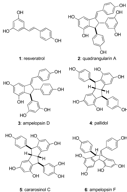
Figure 1. Resveratrol ( 1 ) and some of its derivatives ( 2–6 ).
