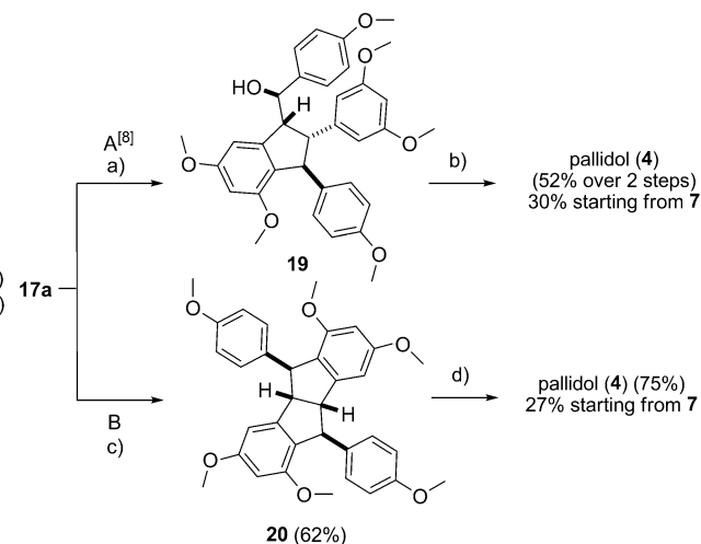
Scheme 4. Total synthesis of pallidol ( 4 ). Reagents and conditions: a) BH 3 ·THF (10 equiv), THF, RT, 18 h, NaOH (0.25 M)/H 2 O 2 (30%) [3:1], 1 h, basic workup; b) BBr 3 (30 equiv), CH 2 Cl 2 , 0 °C/RT, 8 h, 52 % over 2 steps (HPLC purification); c) BH 3 ·THF (10 equiv), THF, RT, 18 h, NaOH (0.25 M)/H 2 O 2 (30%) (3:2), 3 h, aqueous workup, 62%; d) BBr 3 (30 equiv), H 2 O (1 equiv), CH 2 Cl 2 , 0 °C/RT, 8 h, 75 % (FC purification).
